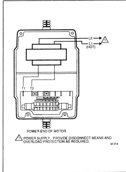
Fig. 1—Mounting 198162 transformer in Modutrol IV motor.
