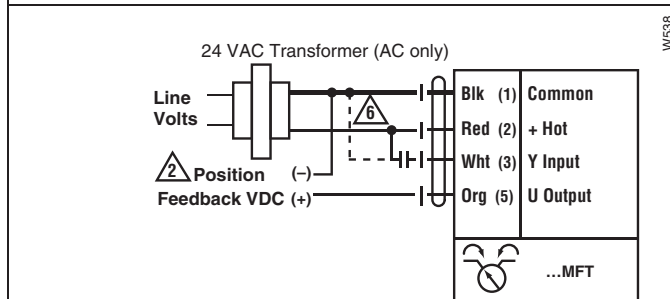
VDC/4-20 mA
