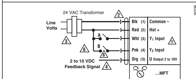
On/Off Control
