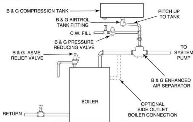
Model EAS with Conventional Compression Tank
