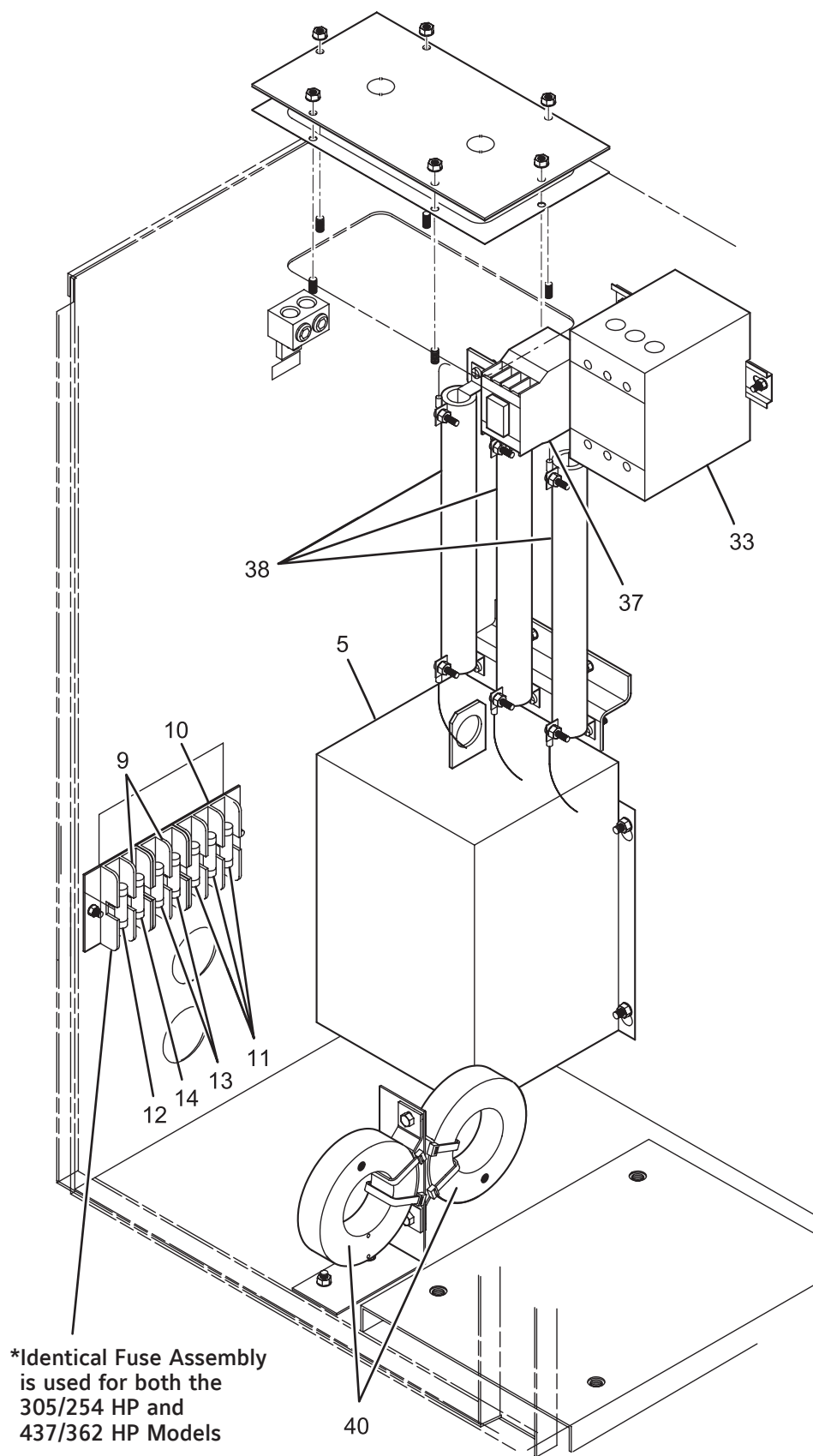
Figure 1. Cabinet, Left Side, 305/254 HP, Typical.
