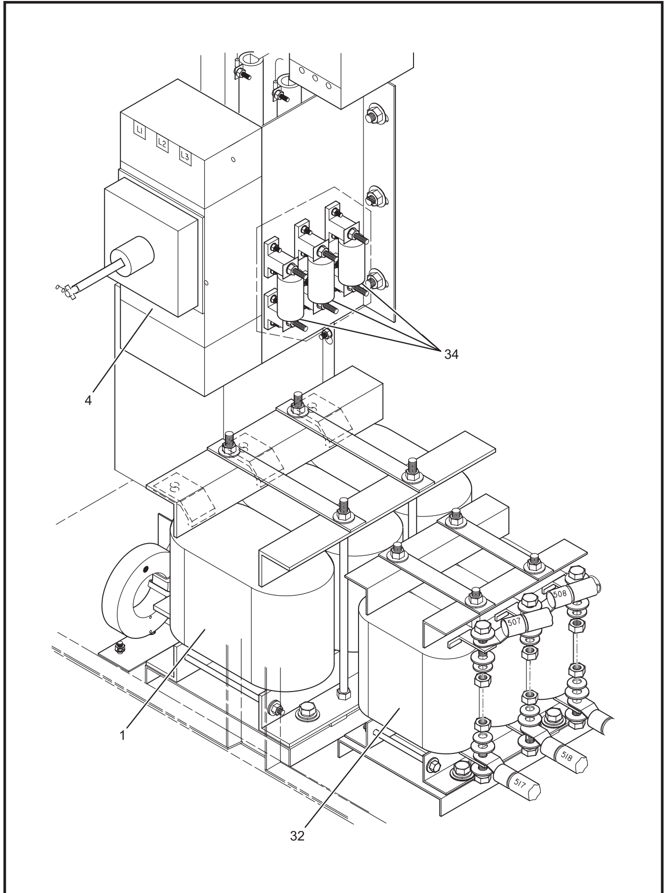
Figure 2. Cabinet, Left Side, 305/254 HP, Typical.
