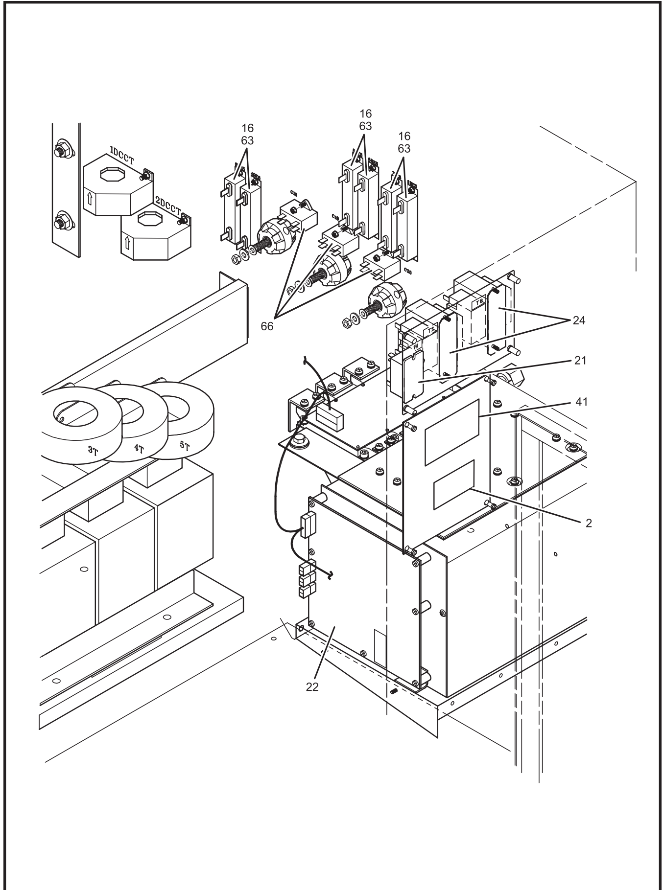
Figure 9. Cabinet, Upper Right Side, 437/362 HP, Typical.
