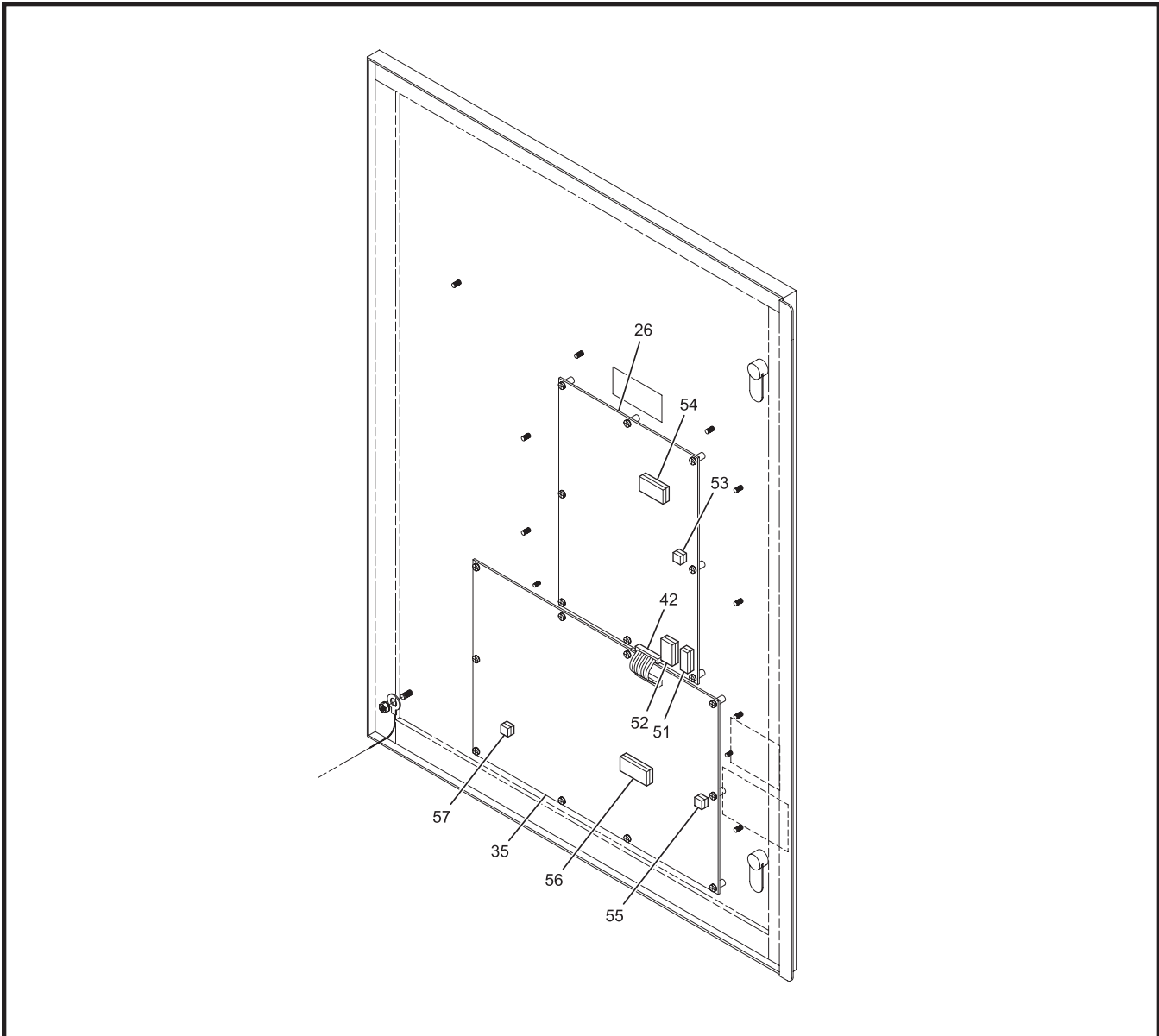
Figure 5. Door, Inside Right, 305/254 HP & 503/362 HP, Typical.
