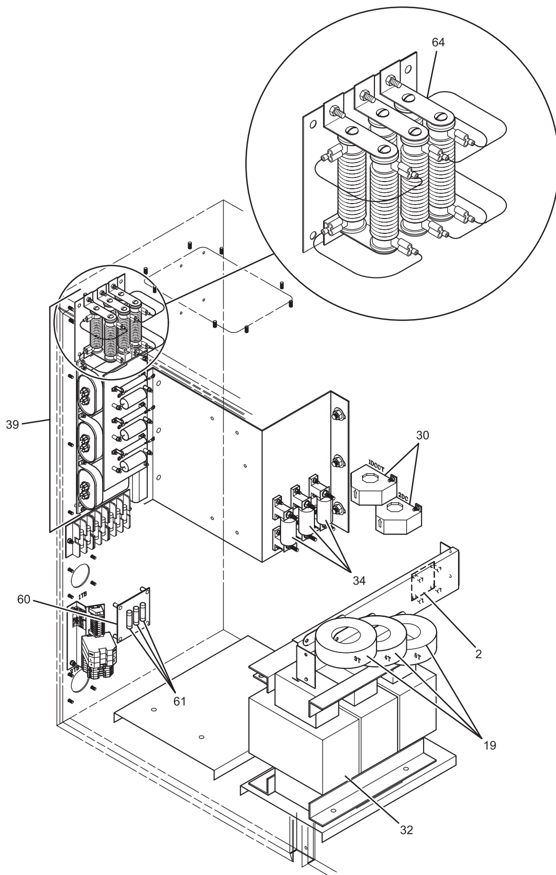
Figure 8. Cabinet, Left/Front Side with Filter Trap Resistor Detail, 437/362 HP, Typical.
