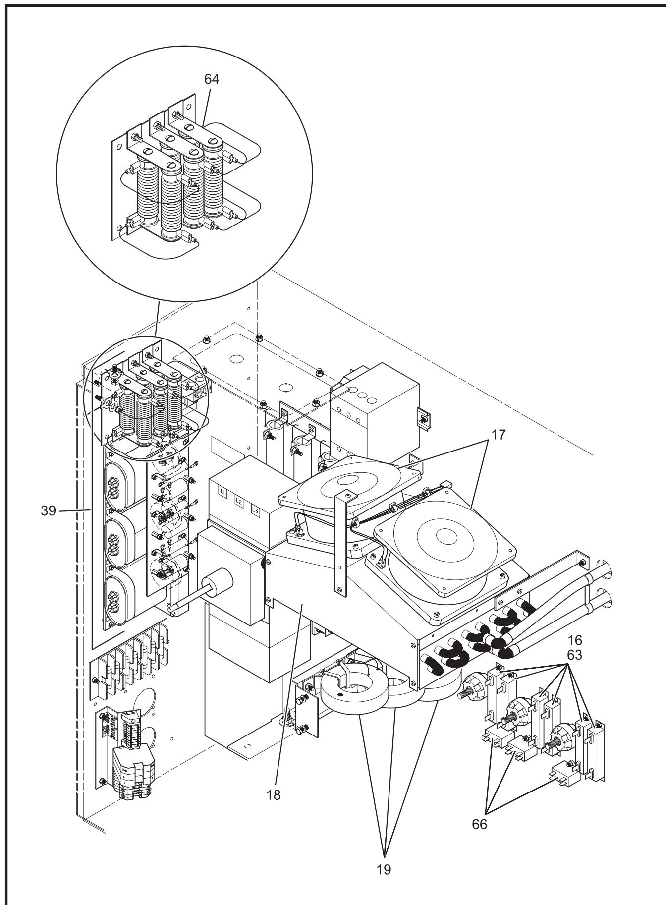
Figure 3. Cabinet, Left/Front Center with Filter Trap Resistor Detail, 305/254 HP, Typical.
