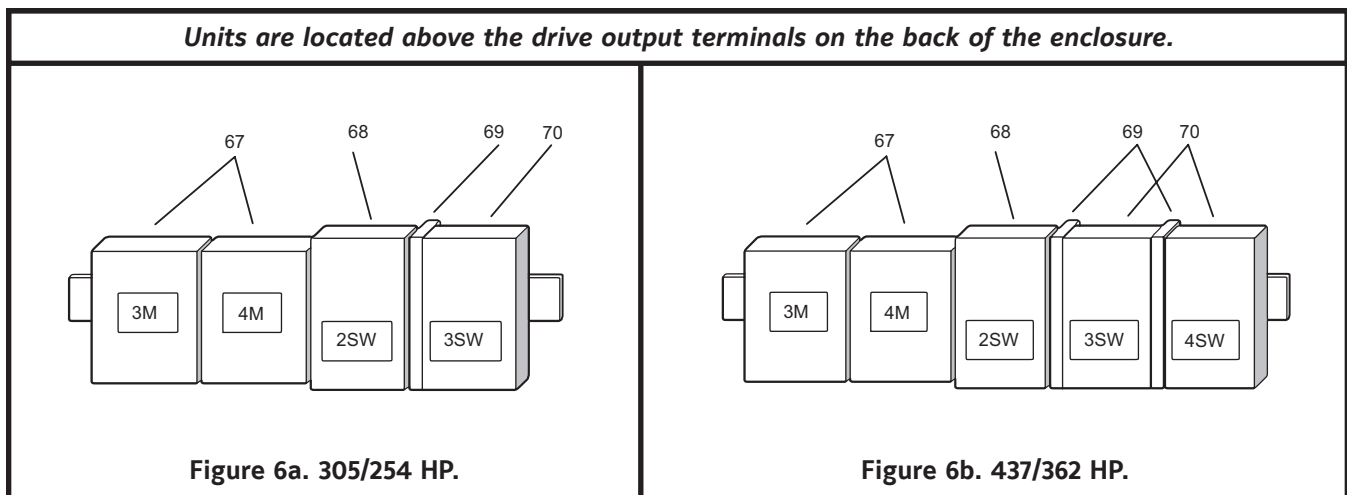
Figure 6. Oil Pump & Blower Motor - Starting Contactors, Overloads & Auxiliary Contact.
