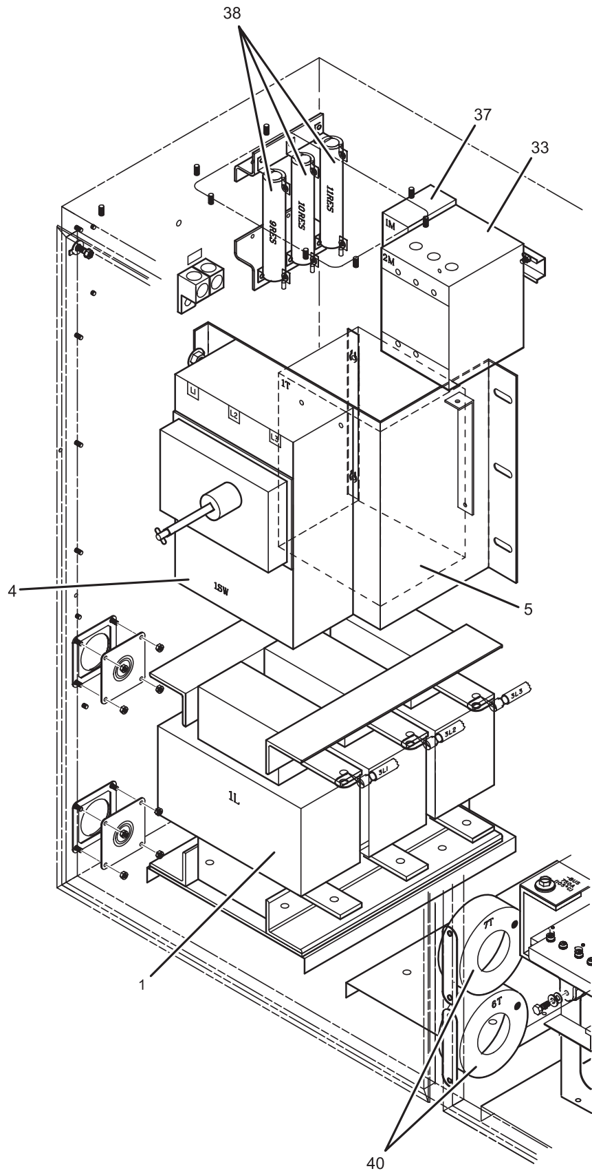
Figure 7. Cabinet, Left/Front Side, 437/362 HP, Typical.
