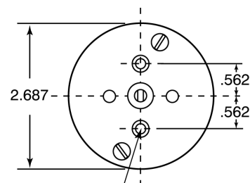
Two Screw Mounting
