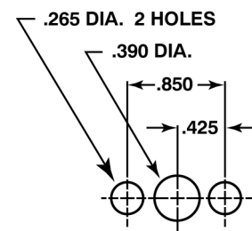
Center Stud Mounting
